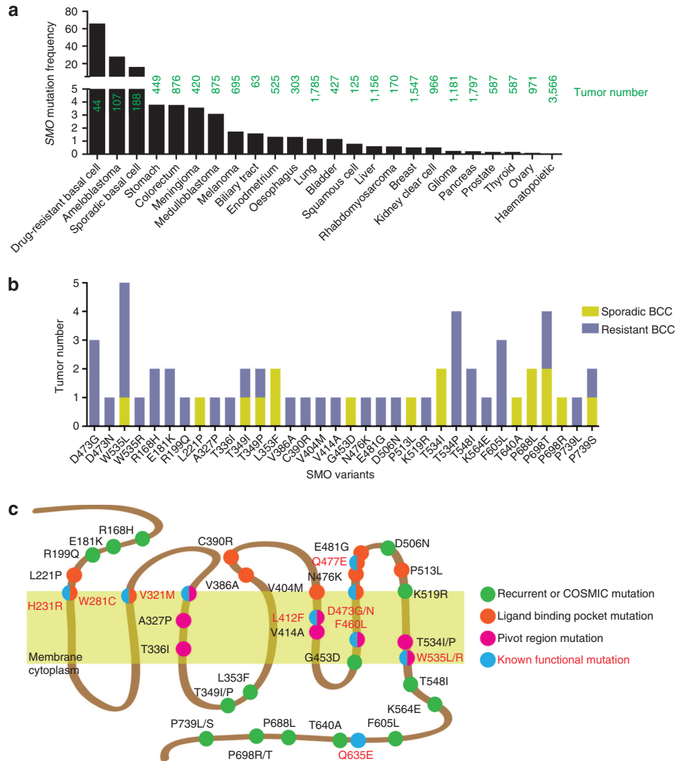
Figure 1. Mutational profile of Smoothed (SMO) in advanced basal cell carcinoma. (a) Frequency of SMO mutations in various cancers seen in the COSMIC database and in current literature (Kool et al., 2014; Lee et al., 2014; Sweeney et al., 2014; Atwood et al., 2015). (b) Number of tumors bearing recurrent, COSMIC database, or region-specific (ligand-binding pocket or pivot region) mutations. (c) Schematic of SMO showing the location of mutations. BCC, basal cell carcinoma.
